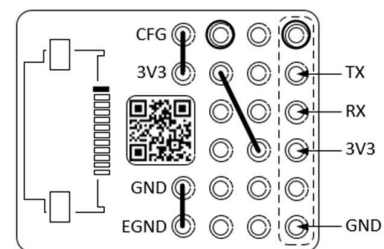
Extra wire jumper RX to CS_N (SYS_WU) to support SLEEP wakeup in UART mode
